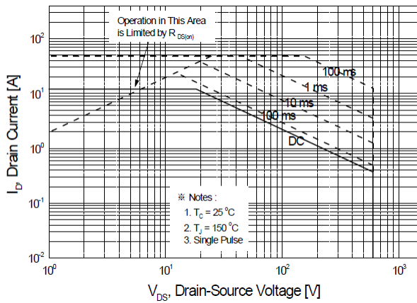
Figure 9-1. Maximum Safe Operating Area for JFPC12N60C
