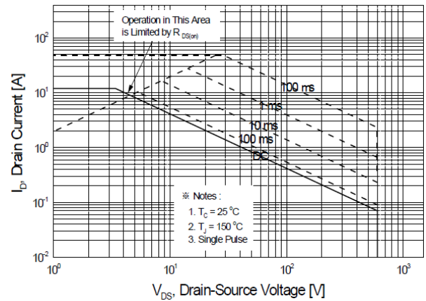
Figure 9-2. Maximum Safe Operating Area for JFFM12N60C
