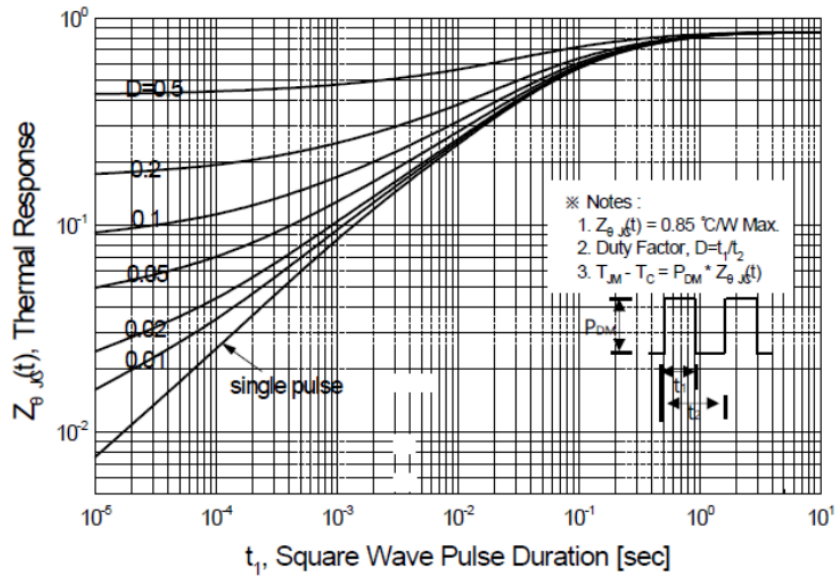
Figure 11-2. Transient Thermal Response Curve for JFPC8N65D
