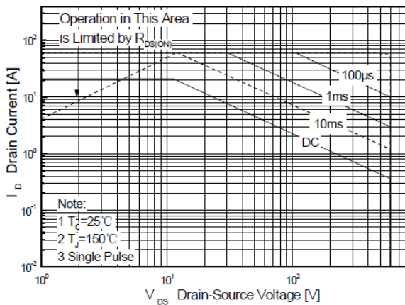
Figure 9-2. Maximum Safe Operating Area for JFPC20N65C
