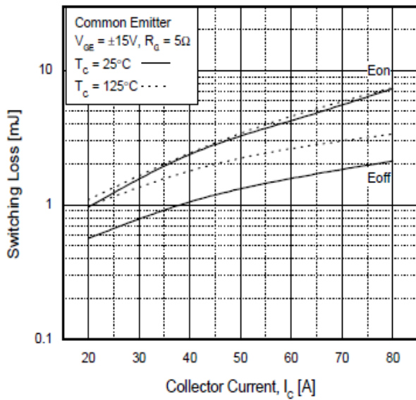
Figure9: typical energy loss VS. I_C , T_C=25^\circ C , L=500\mu H , V_{CE}=600V , V_{GE}=15V , R_G=5\Omega
