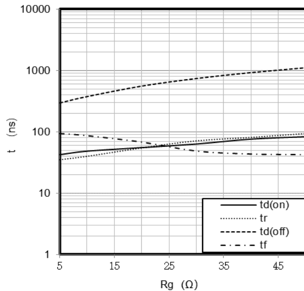
Figure12: typical switching time VS. R_G , T_C=25^\circ C , L=500\mu H , V_{CE}=600V , V_{GE}=15V , I_C=20A
