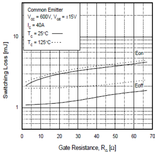
Figure11: typical energy loss VS. R_G , T_C=25^\circ C , L=500\mu H , V_{CE}=600V , V_{GE}=15V , I_C=40A
