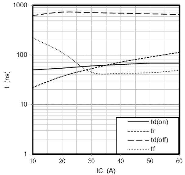
Figure10: typical switching time VS. I_C , T_C=25^\circ C , L=500\mu H , V_{CE}=600V , V_{GE}=15V , R_G=28\Omega
