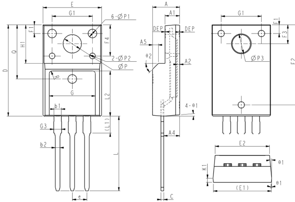
COMMON DIMENSIONS
