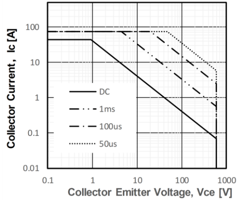
Figure 14. SOA Characteristics
