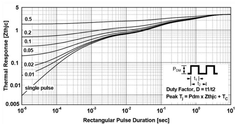
Figure 19. Transient Thermal Impedance of IGBT
